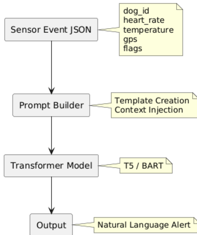
Figure 2: Multi-sensor data to natural language alert: transformation pipeline.
